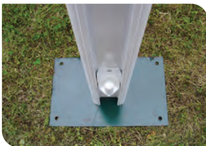
Posts slot onto a green steel base plate for stability. Base plates have pre-drilled holes to allow for extra staking into soft ground.
